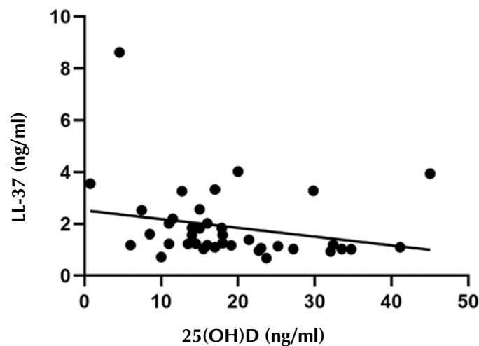
Figure 4. Relationship between serum 25-hydroxyvitamin D and cathelicidin (LL-37) in S. aureus nasal carriers. There was a moderate negative correlation between 25(OH)D and LL-37 in nasal carriers (coefficient = -0.392, p = 0.011 ).
